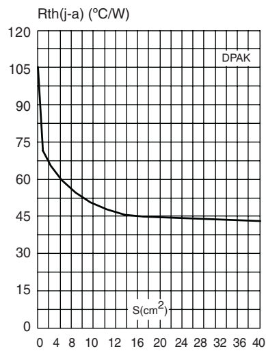
Fig. 9: DPAK Thermal resistance junction to ambient versus copper surface under tab (printed circuit board FRA, copper thickness: 35µm).
