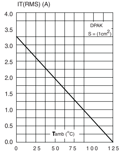
Fig. 8: DPAK RMS on-state current versus ambient temperature (printed circuit board FR4, copper thickness: 35µm), full cycle.
