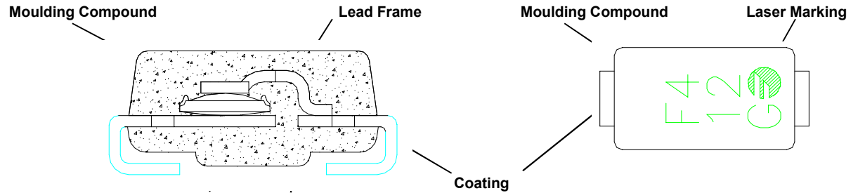
Lead Frame
