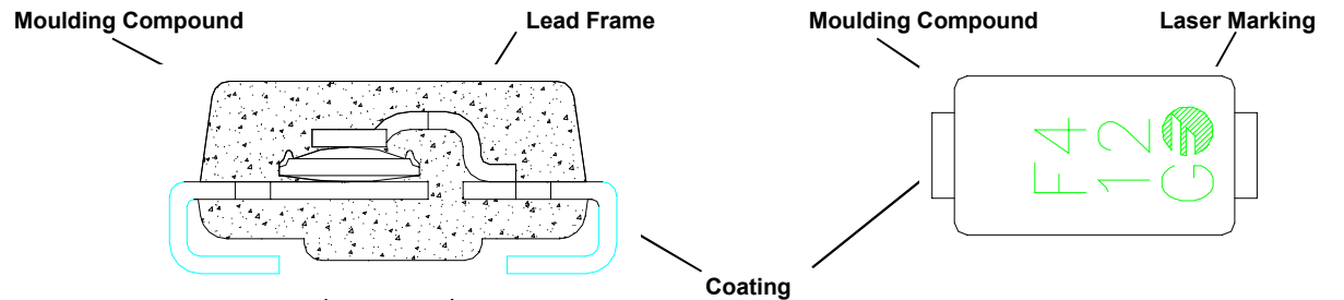
DIODE DRAWING
