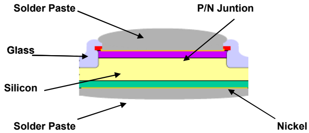
CHIP DRAWING
